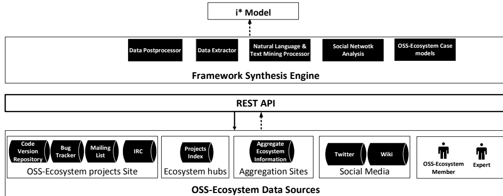
Fig. 2. OSS-Ecosystem Model Synthesis
