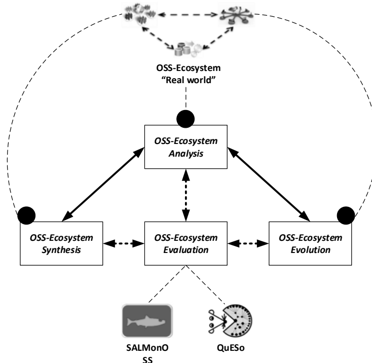
Fig. 1. OSS-ecosystem modelling framework
