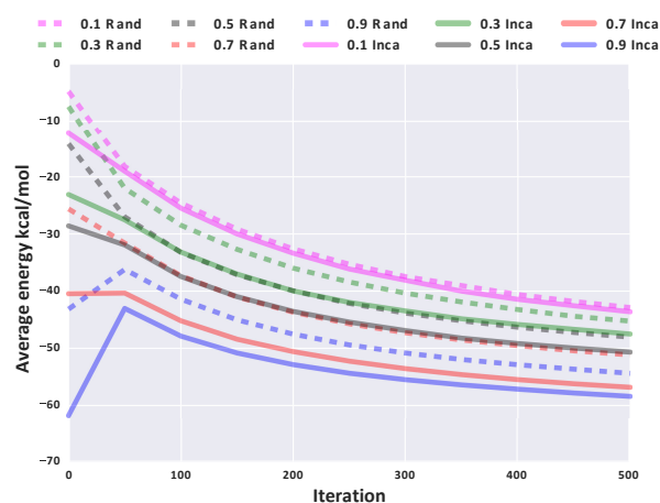
Figure 4. Comparison of the free-energies of candidate solutions along the execution of RNAfbinv, for targeted GC contents from 0.1 to 0.9 and using incARNAtion (solid lines) and the default random initialization of RNAfbinv (dashed lines), for the design of a guanine-binding riboswitch aptamer. Values averaged over 1000 runs.
