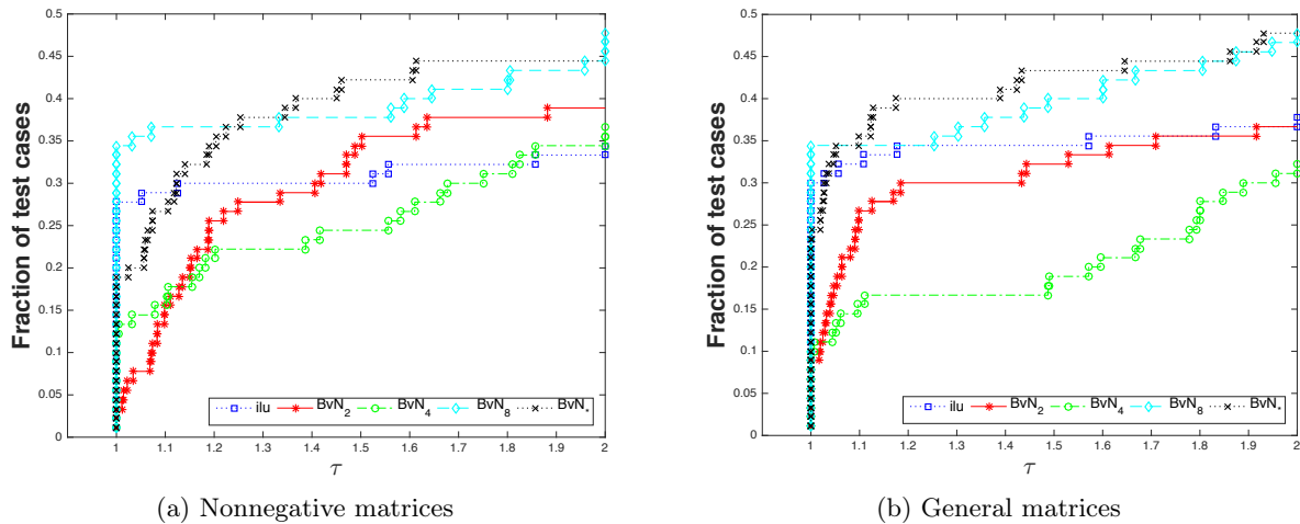
Figure 1 – Performance profiles for the number of iterations with ILU(0), BvN r with r = 2, 4, 8 , and BvN * .
