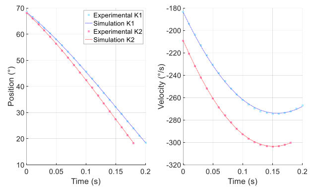
Figure 2: Experimental and simulation knee kinematics (angular position and velocity) for both stiffness settings.
