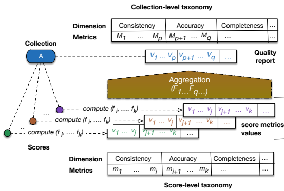
Figure 3. Metrics computation
