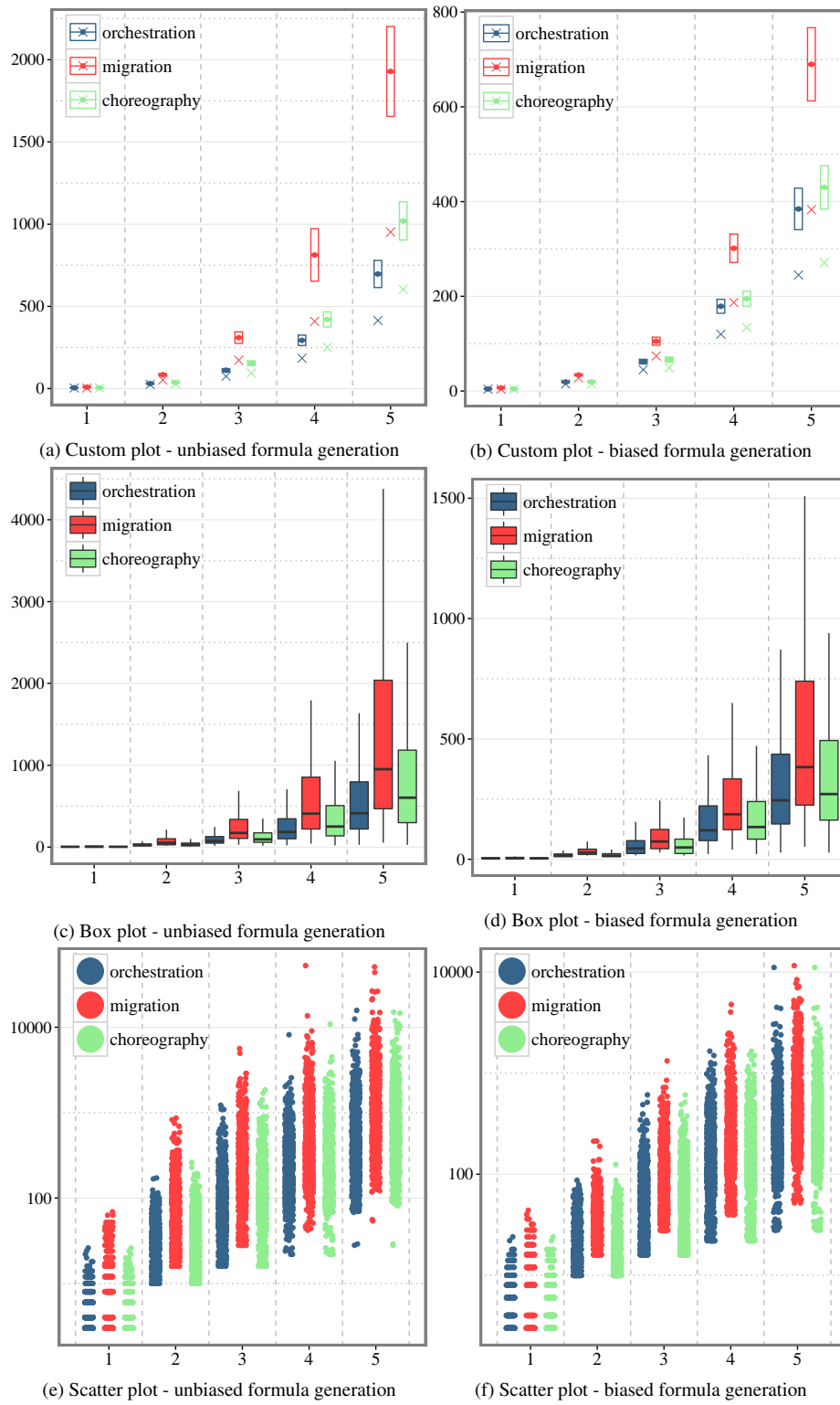
Fig. 9: Visualisation of the results (reported in Table 2) obtained for the number of progressions ( \#prog in ordinate with the experiment varying the size of formulae ( |\varphi| in abscissa)). A base-10 logarithmic scale is used for the ordinate axis of scatter plots.
