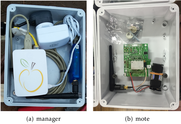
Figure 5. The devices encased in 20 cm × 15 cm IP65 enclosures.
