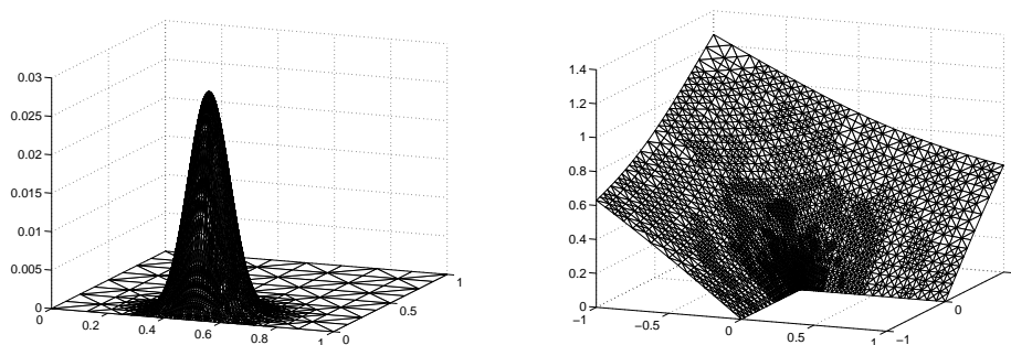
Figure 1: Left: solution (7.1) of the peak problem. Right: solution (7.2) of the L-shape problem.
