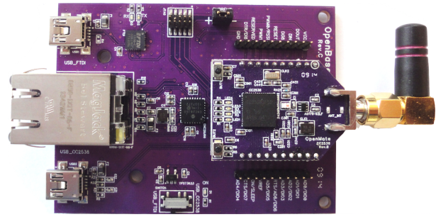
Fig. 2. An OpenMote-CC2538 and an OpenBase board.
