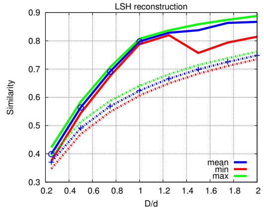
Figure 4: Reconstruction from LSH: a(\mathbf{x}) as a function of D/d . Empirical mean, min. and max. over 10,000 reconstructions. Unif. Tight Frame (plain), Gaussian i.i.d. (dashed), Eq. (8) (+) and Eq. (9) (o).
