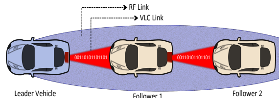
Fig. 1. VLC used for intra-platoon communications.
