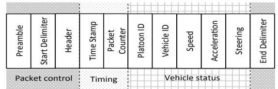
Fig. 3. Packet format for intra-platoon communication.
