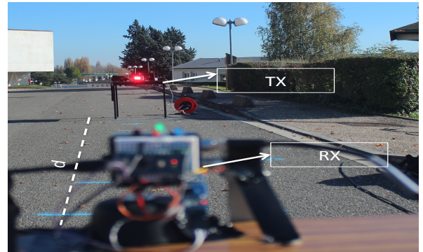
Fig. 5. Experimental setup
