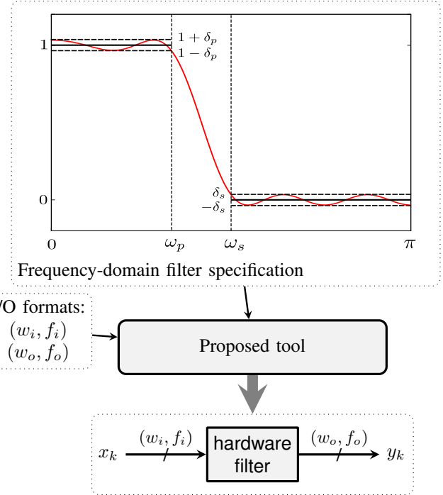
Fig. 1: Generating a hardware digital filter out of a minimal specification (here on a generic low-pass filter defined by passband frequency \omega_p , stopband frequency \omega_s , and bounds \delta_p and \delta_s on the passband ripple and stopband attenuation).
