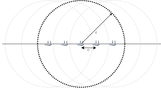
Figure 3: Radio coverage of access nodes (ANs) in linear access networks. ANs are placed every c meters and have a radio coverage of r meters.
