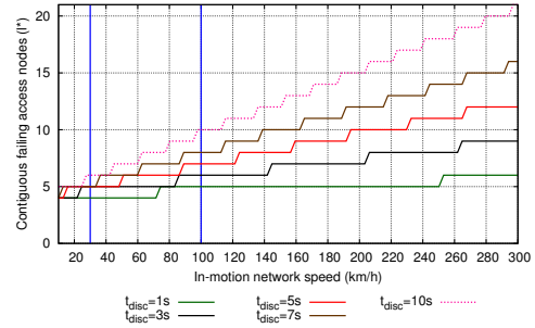
Figure 5: Maximum number of contiguous failing access nodes that the network can tolerate, l^* , as a function of the vehicle speed for different values of t^* , the maximum disconnection time tolerated.
