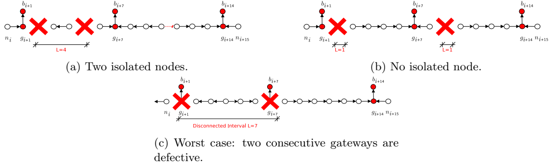
Figure 2: Different cases of isolated nodes produced by two defective nodes.
