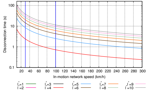
Figure 4: Disconnection time (log-scale) for different speeds and different number of failed nodes.
