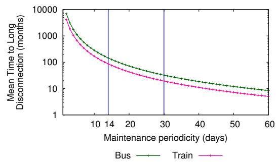
Figure 12: Mean time to a long disconnection for the linear access network as a function of the periodicity of the network maintenance.
