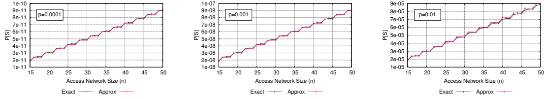
Figure 10: Validation of the approximation formula for different values of p , the probability of failure of an access node.
