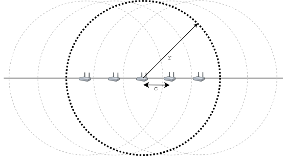
Figure 3: Radio coverage of access nodes (ANs) in linear access networks. ANs are placed every c meters and have a radio coverage of r meters.
