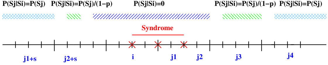
Figure 7: Syndrome dependence: \mathbb{P}[S^j|S^i] \leq \mathbb{P}[S^j]/(1-p) .
