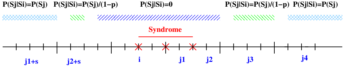
Figure 7: Syndrome dependence: \mathbb{P}[S^j|S^i] \leq \mathbb{P}[S^j]/(1-p) .
