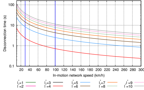
Figure 4: Disconnection time (log-scale) for different speeds and different number of failed nodes.
