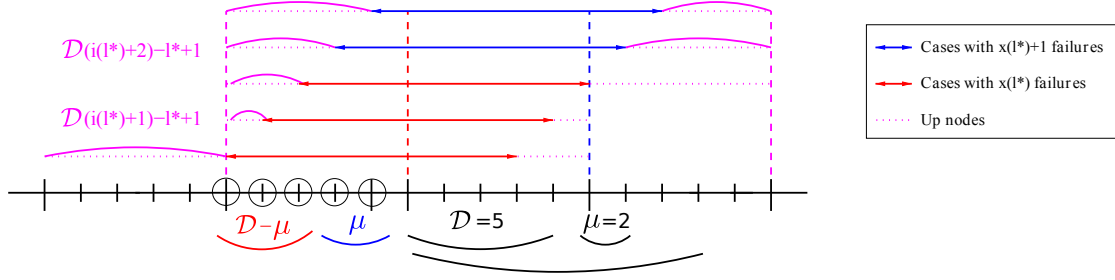
Figure 8: Sketch of the proof for a syndrome
