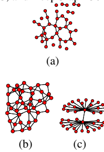
Figure 2: Example of (a) random (b) small world (c) hub networks used in experiments
