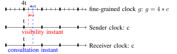
Fig. 4. Example of advance nodes defines on a fine-grained clock.
