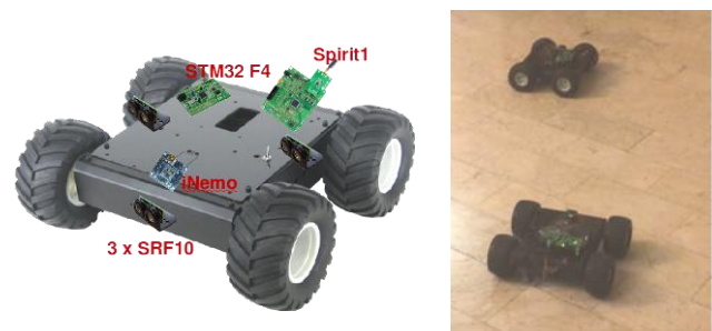
Figure 4. The cooperating robots during an experiment.
