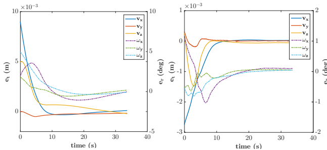
Fig. 6. Positioning task [simulation case]: (left) error decay in each DOF and (right) velocity evolution in each DOF.
