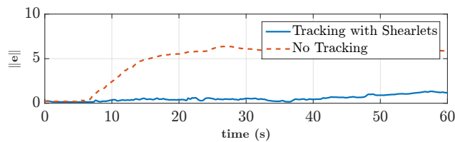
Fig. 12. Evolution of the error in the Shearlet domain for different tracking commands.
