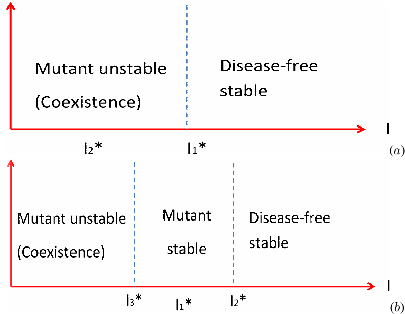
Figure 2: Regions of stability of impulsive orbits. When I_2^* < I_1^* , if I > I_1^* , the disease-free orbit becomes stable and the mutant cannot survive on its own (see Fig. 2 (a)). Conversely, if I < I_1^* , both strains coexist. If I_2^* > I_1^* The disease-free orbit is stable if I > I_2^* and unstable otherwise. When I_3^* < I < I_2^* , the mutant survives on its own, while if 0 \leq I < I_3^* , both strains coexist.
