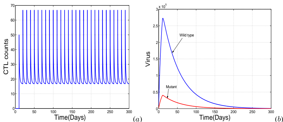
Figure 3: When the vaccine is taken every ten days, stimulating 50 cells/1L, CTL cells converge to an impulsive periodic orbit (Fig 3.(a)); if the vaccination frequency is increased, then we have eradication of both strains (Fig 3.(b)).
