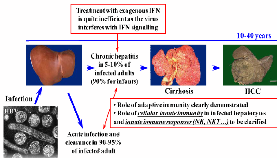
Figure 1: Natural history of HBV infections. HCC, hepatocellular carcinoma; NK, natural killer cells; NKT, natural killer T cells.
