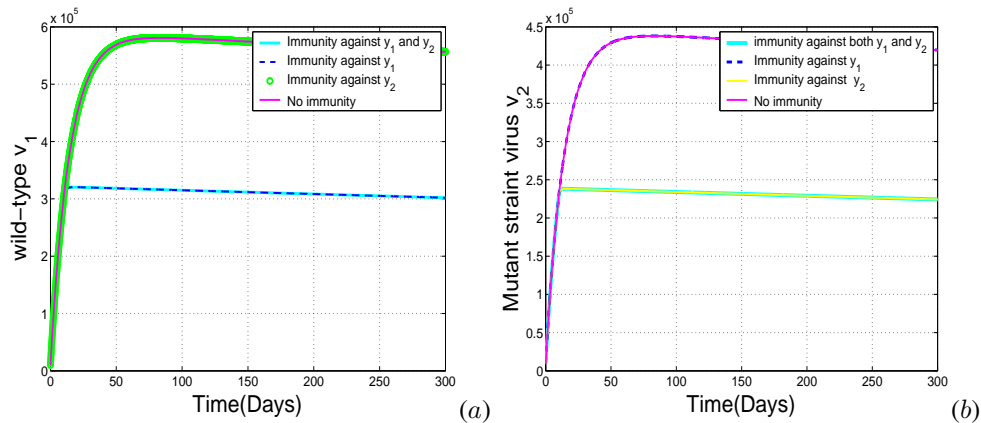
Figure 5: 0 \leq I < I_3^* , d_v = 0.00021 and the two populations coexist (Fig.5 (a)) and Fig.5. (b). The two strains population exist. The target of immune response strongly influences the outcome of infection in HBV model with two strains.
