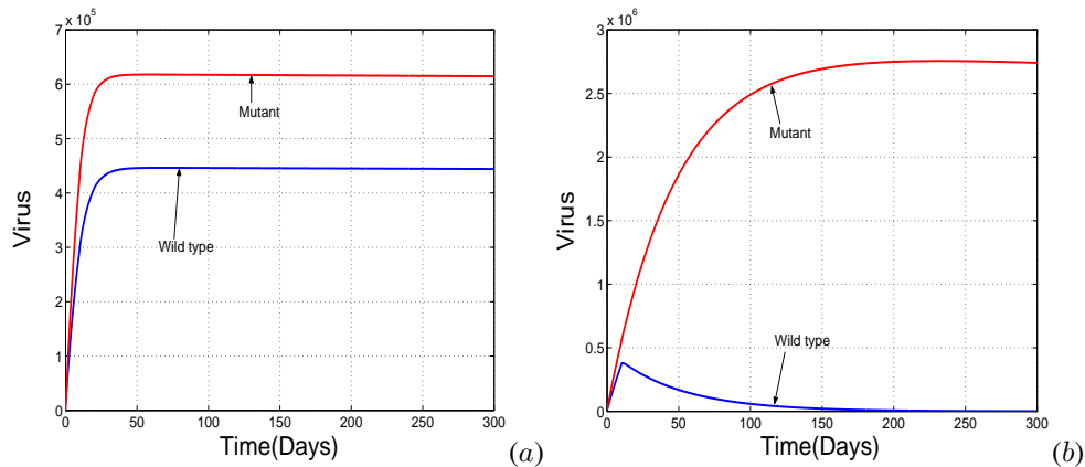
Figure 4: 0 \leq I < I_3^* , d_v = 0.00021 and the two populations coexist (Fig.4 (a)). The mutant exists at high levels (approximately 2.7 \times 10^6 virions/1L), but the wild type is eradicated. This one is obtained when I_3^* < I_2^* (Fig.4.(b)).
