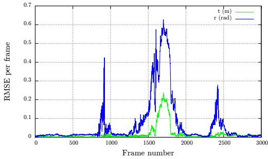
Figure 13: Error to ground truth for the CPU-based approach on the second sequence.
