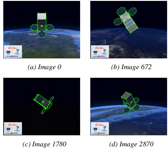
Figure 10: Vision-based navigation of a CubeSat at 400km altitude (approximately ISS altitude), using the GPU-based approach.
