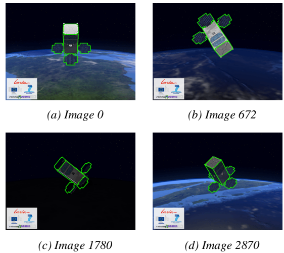
Figure 11: Vision-based navigation of a CubeSat at 400km altitude (approximately ISS altitude), using the CPU-based approach.
