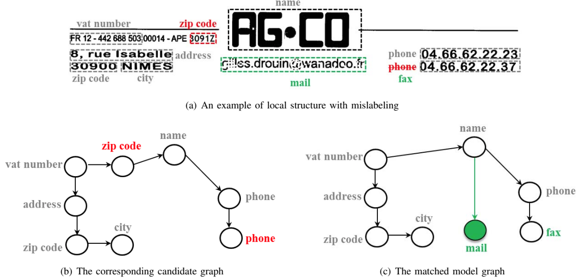
Fig. 3. Mislabeling correction in a local structure using subgraph matching
