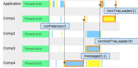
Fig. 6. Code execution
