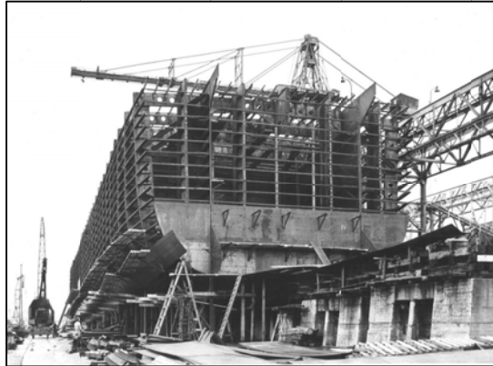
Fig. 2. Building Berth on Old Shipyard
