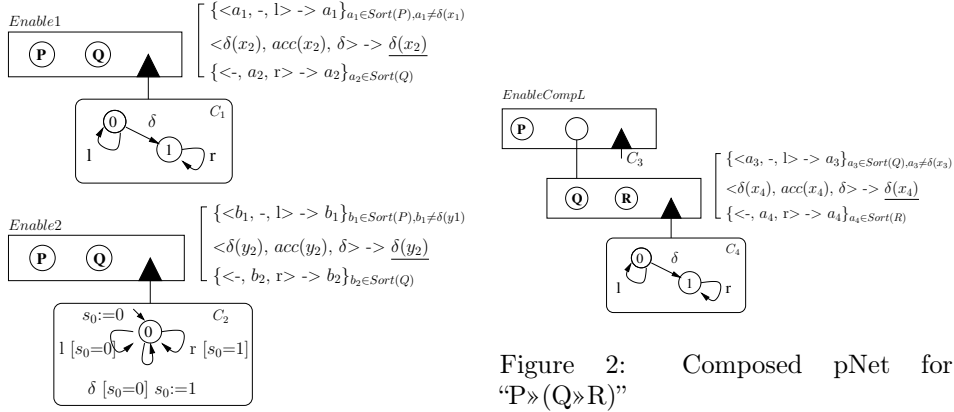
Figure 1: Two pNet encodings for Enable
