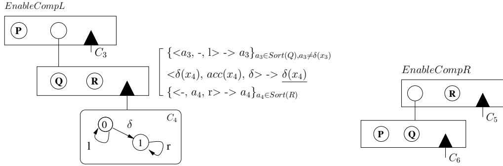
Figure 5: Structure of the pNets for “ P \gg (Q \gg R) ” and “ (P \gg Q) \gg R ”
