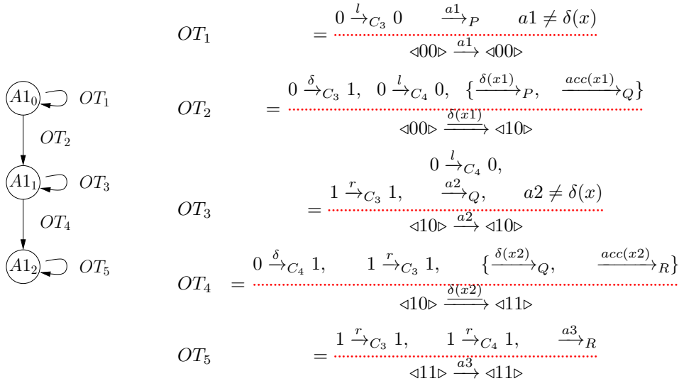
Figure 6: Open Automaton for the term “ P \gg (Q \gg R) ”
