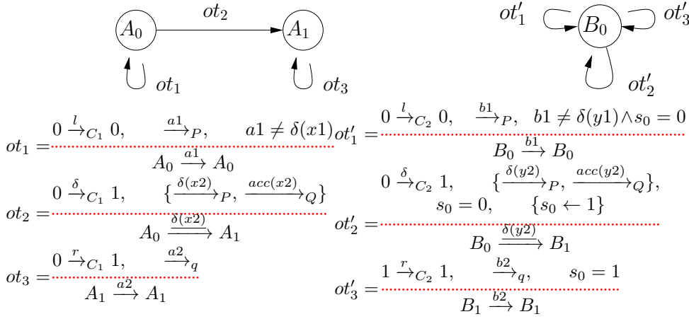
Figure 4: The two open automata
