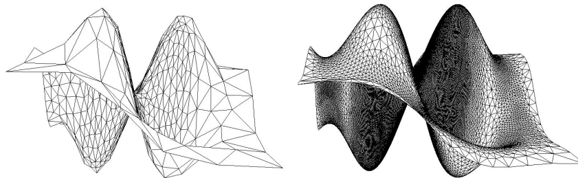
Figure 4. approximate pressure. On the left, the first iteration with 467 DOF, on the right the last iteration with 5667 DOF.
