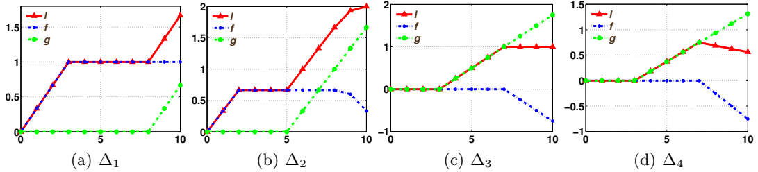
Figure 3: The plot of the four loss functions used in our experiments as in Equations (33) to (36). The x axis is the number of mispredictions for each track (we show here the loss functions corresponding to track length equal to 10 as an example), and the y axis is the value of loss function. The original losses are drawn in red; the supermodular components are drawn in green, and the submodular components in blue.
