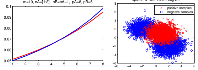
Figure 1: Plots of Eq. (31) Figure 2: The data (red) and Eq. 32 (blue) as a for the synthetic problem of n_A . As these two lem. The negative samples are drawn from a mixture of Gaussians. plots cross, neither function bounds the other.
