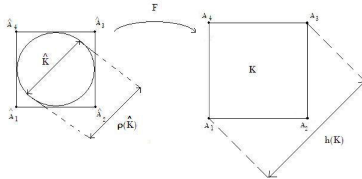
Figure 3. The mapping F .
