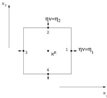
Figure 1. The Raviart-Thomas H(\operatorname{div}, \Omega) first order finite element
