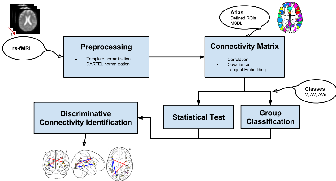
Fig. 3. Proposed pipeline for analyzing rs-fMRI data from pre-processings (temporal and spatial including normalization using DARTEL in SPM12) to supervised classification (binary group comparisons like AV-V ). The outcome of supervised classification allows us to unravel the discriminant functional interactions between groups. This pipeline was implemented in Python language using the nipype interface and the nilearn software ( http://nilearn.github.io/ ).
