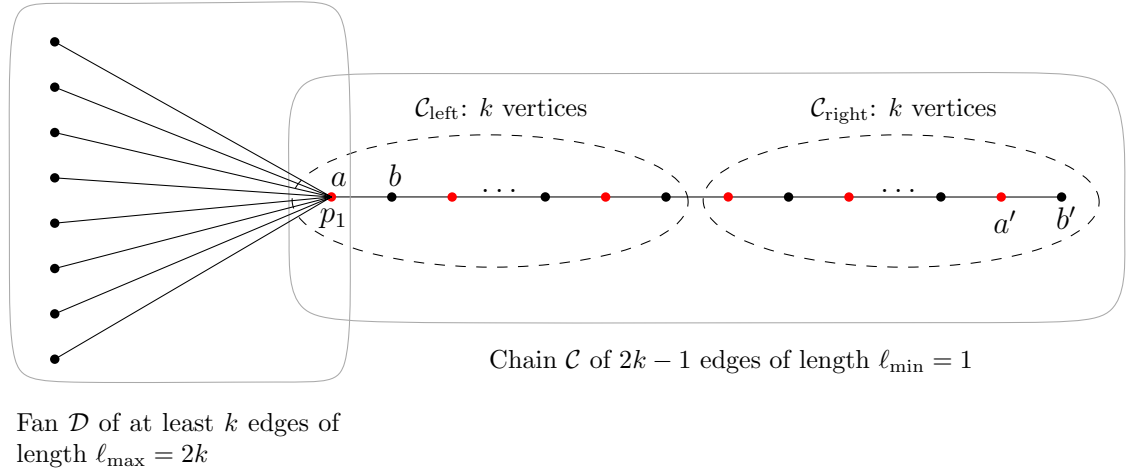
Figure 2: Graph \mathcal{G} for which \mathcal{F}_{FPS} \geq \frac{1}{2}r_e\mathcal{F}^* .
