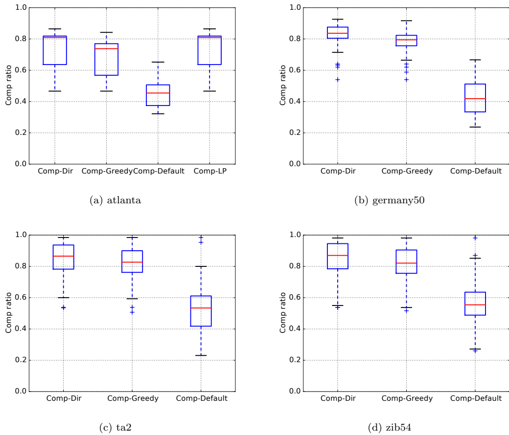
Figure 6: Compression ratio of the three different heuristics on 4 different SNDlib topologies.
