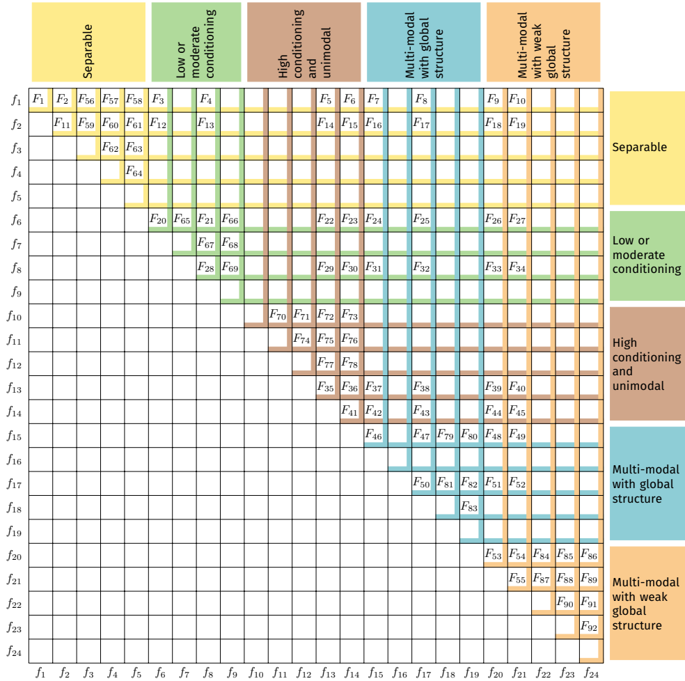
Figure 2: The functions of the bbob-biobj-ext test suite ( F_1 to F_{92} , in the table cells) together with the information about which single-objective bbob functions are used to define them (left and bottom annotations).
