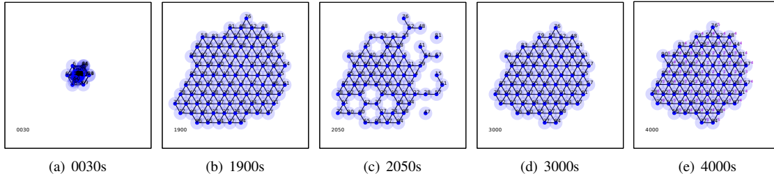
Fig. 9: EMR algorithm presented in this paper. Deployment snapshots with 30% of node disappearing at 2000s and the self-healing mechanisms.
