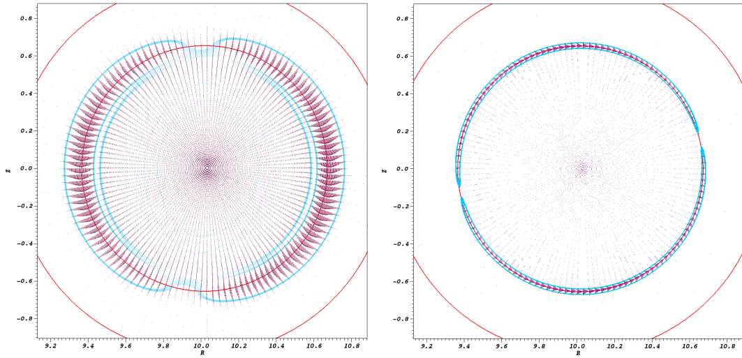
Figure 5: Kink structure comparison for S = 10^5 (left) and S = 10^8 (right). The width of the structures depends on the Reynolds Magnetic number. Going from 10^{-1} (left) to 3 \cdot 10^{-2} (right)
