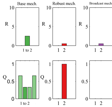
Figure 13: Robust mechanism, optimized and broadcast schemes minimizers in example C.3.
