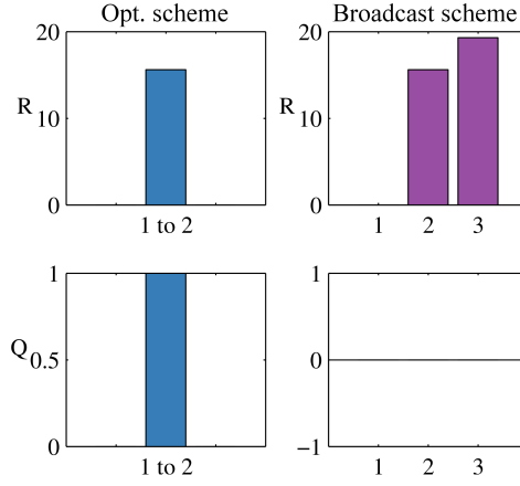
Figure 9: Optimized and broadcast schemes minimizers in example C.1.
