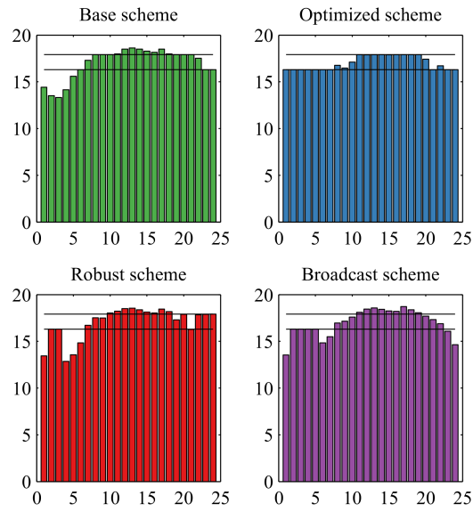
Figure 2: Final consumption in GWh for the four DR mechanisms ( \mu = \frac{1}{10} ). The black lines represents respectively C_1 and C_2 .
