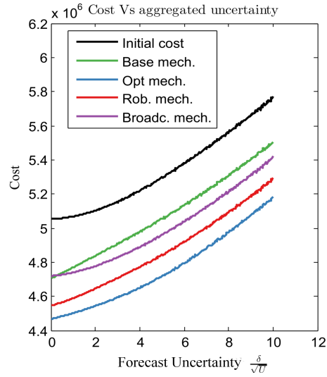
Figure 6: Global cost versus relative uncertainty \frac{\delta}{\sqrt{U}} (%).
