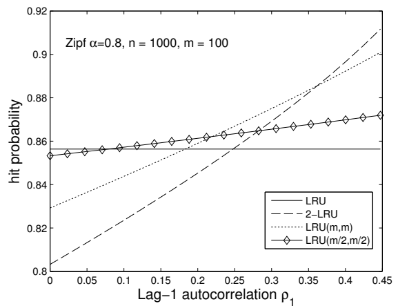
Fig. 4. Hit probability as a function of the lag-1 autocorrelation \rho_1 for LRU, LRU(m, m) , LRU(m/2, m/2) and 2-LRU when subject to MAP arrivals (with z = 10 ).
