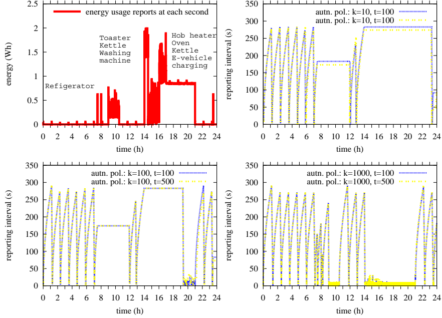
Fig. 1. Raw energy usage over time, at the left top and autonomically adapted intervals.
