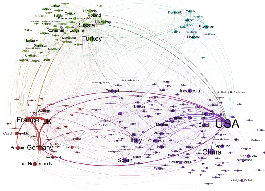
Fig. 2. Country network: node size corresponds to degree and node colours indicate the four clusters obtained with the Louvain method.
