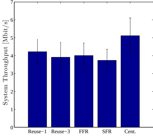
Fig. 5: System throughput
