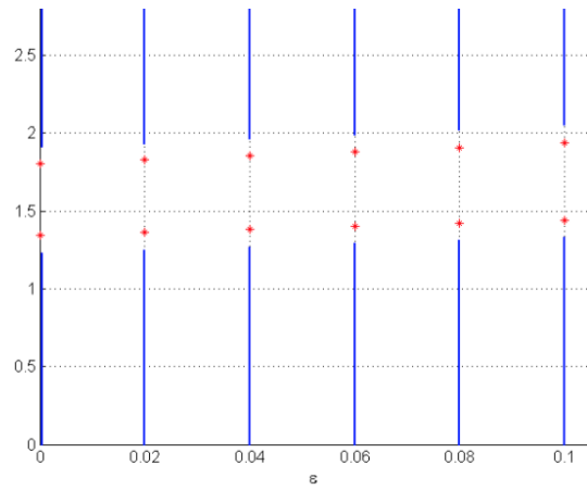
Figure 12: Representation of the eigenvalues appearing in the first gap of the operator A_{\epsilon,s}^\mu for different values of \epsilon for L = 2 and \mu = 0.25 (red asterisks). The values for \epsilon = 0 correspond to the limit operator A_s^\mu .
