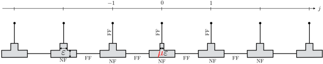
Figure 10: Schematic representation of the asymptotic expansion (NF: near field, FF: far field).
