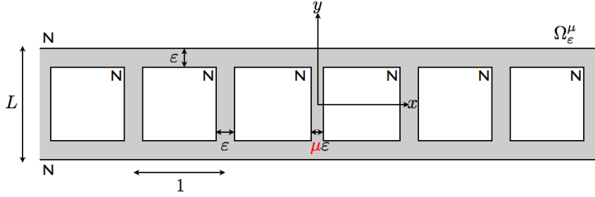
Figure 2: The Perturbed ladder
