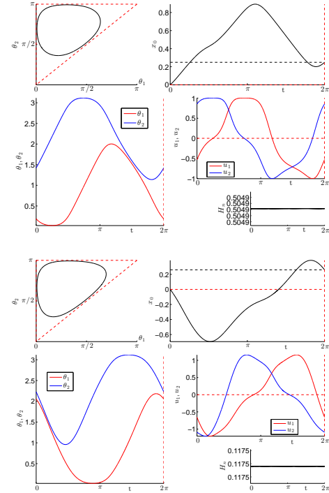
Fig. 12. Normal stroke for the \int_0^{2\pi} (u_1^2 + u_2^2) dt cost (top) and the mechanical cost (bottom) where the constraints are satisfied (simple loop).
