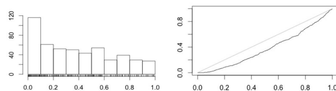
(c) n = 500 , under H_0 , well separated clusters
