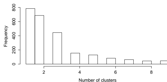
Figure 7: Histogram of the numbers of clusters. They are obtained after applying our clustering method on each sample.
