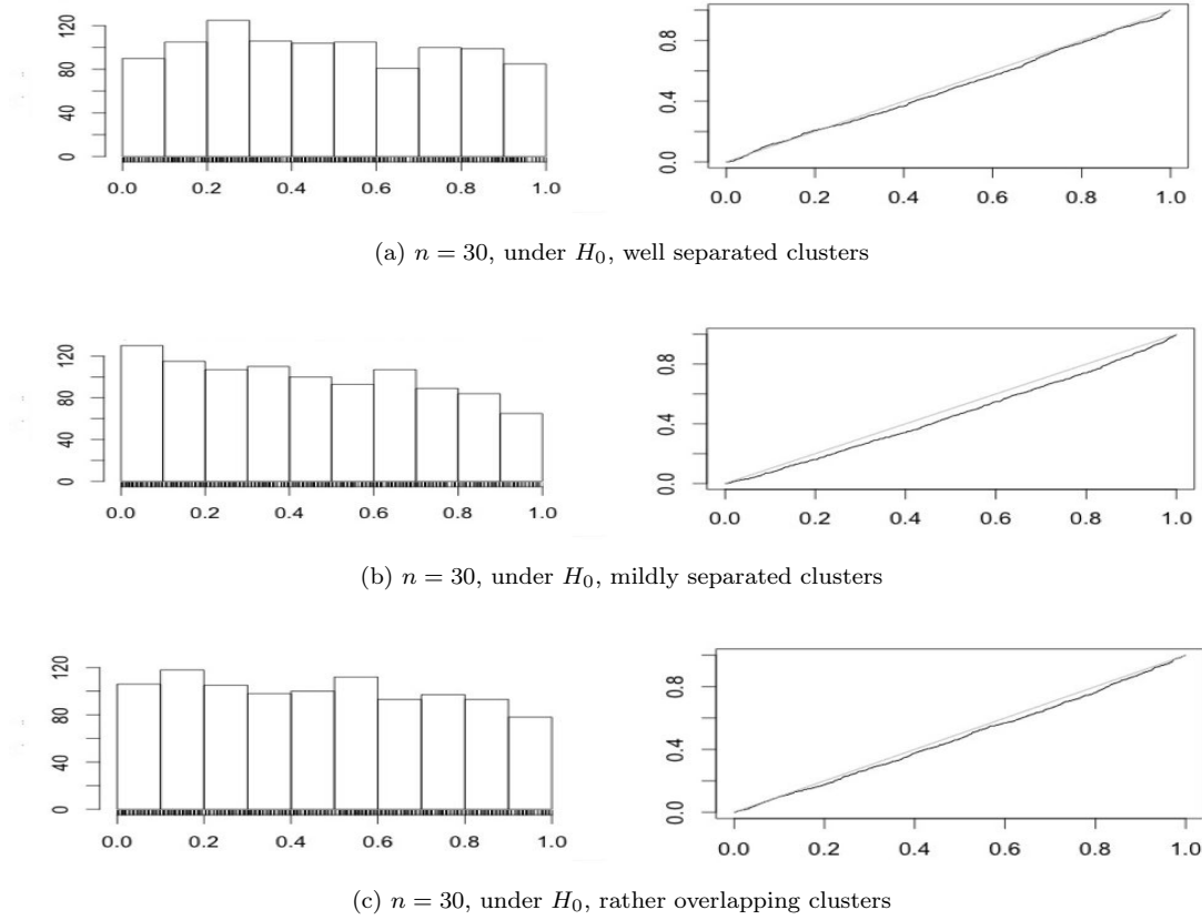
Figure 10: Histogram and QQ-plot of the N = 1000 p -values generated under a GM model, for n = 30 and under 3 possible levels of overlapping of clusters: a uniform distribution is expected for a good calibration of the test (for the QQ-plot, uniformity means being very close to the diagonal line)
