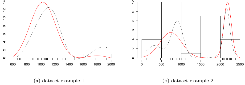
Figure 18: Examples of two datasets of size n = 30 , represented with their histogram, their true underlying GM distribution pdf (in dotted line), and their estimated GM distribution pdf (in solid line) , the individual data values being indicated by ticks on the horizontal axis
