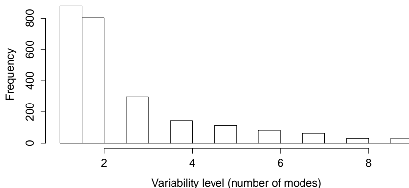
Figure 19: Variability levels of programs executions times
