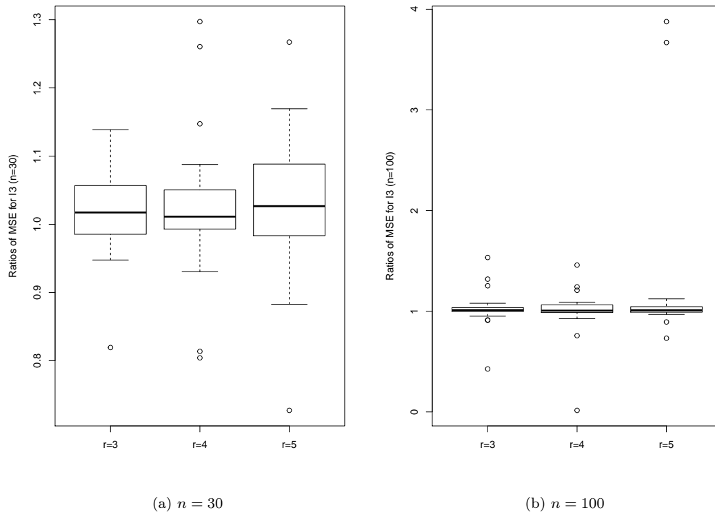
Figure 17: Ratios between the MSE of parametric vs. non parametric estimators of \mathcal{I}_3
