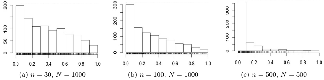
Figure 12: Histograms of the p -values generated under a non GM model (a mixture model of shifted exponentials), for n = 30 , 100, or 500: the capacity of the test to detect that H_0 does not hold, called the power, is measured by the fact that the distribution of the p -values is more concentrated on the vicinity of 0.
