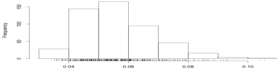
Figure 9: Histogram of the values KS^{(1)} \leq \dots \leq KS^{(N)} for N = 500 for Example 5.1
