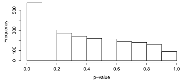
Figure 14: Histogram of the p values. They are obtained after applying our test of fitting using Kolmogorov-Smirnov distance with bootstrap calibration.
