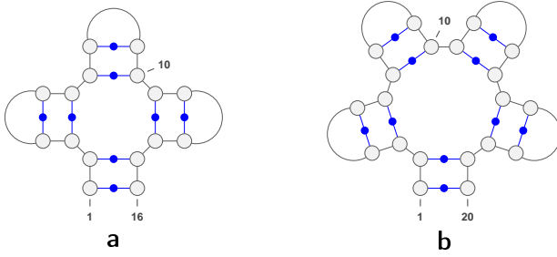
Fig. 4 Examples of two saturated structures, one satisfying conditions of R4 (a.) and one that does not (b.). The structure on the left has pair degree 4 and is designable, and the structure on the right has pair degree 5 and is not designable.
