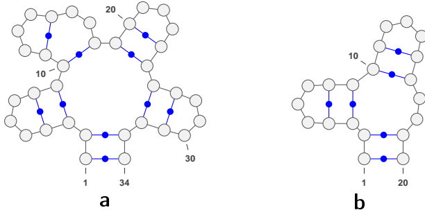
Fig. 5 Examples of two structures containing motifs m_5 (a.) and m_{3 \circ} (b.), respectively. By R5 these two structures are not designable.
