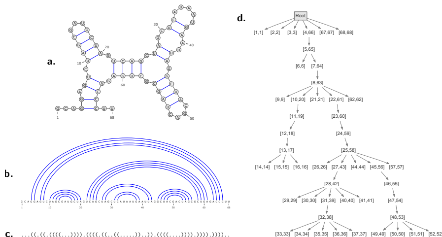
Fig. 1 Four equivalent representations for an RNA secondary structure of length 68, consisting of 20 base pairs forming 7 bands: outer-planar graph (a), arc-annotated representation (b), parenthesized expression (c), and tree representation (d)
