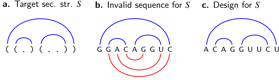
Fig. 2 The combinatorial RNA design problem: Starting from a secondary structure S (a.), our goal is to design an RNA sequence which uniquely folds, with maximum number of base pairs, into S . The sequence proposed in b. is invalid due to the existence of an alternative structure (lower half-plane, red) having the same number of base pairs as S . The right-most sequence (c.) is a design for S .
