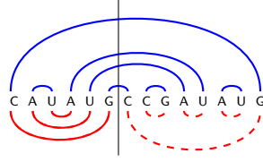
Fig. 5 Construction of the saturated structure compatible with the suffix v . The vertical line splits the sequence into a prefix u and a suffix v . Blue and red arcs depict saturated structures compatible with w and u respectively. Dashed red arcs represent the induced saturated structure compatible with v .
