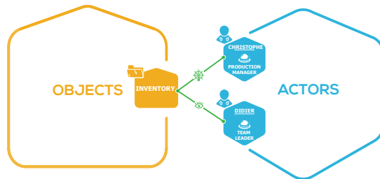
Fig. 6. Pairwise relationships
