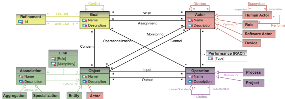
Fig. 1. CHOOSE metamodel [7]
