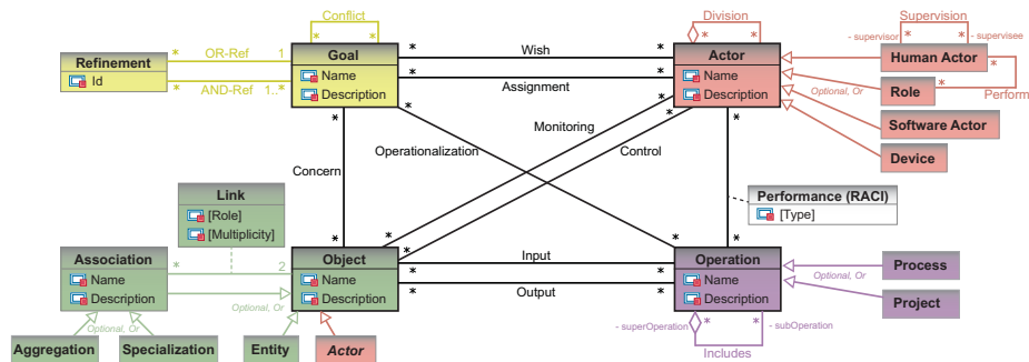
Fig. 1. CHOOSE metamodel [7]
