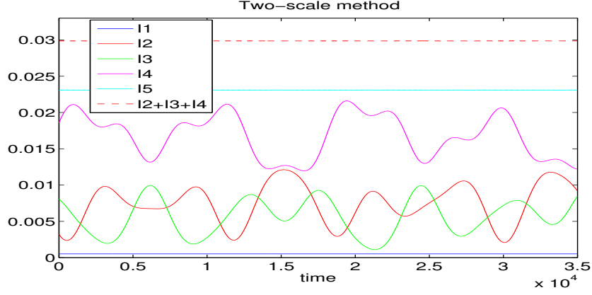
Figure 3: (FPU, d = 1 ) Energy exchanges, two-scale method
