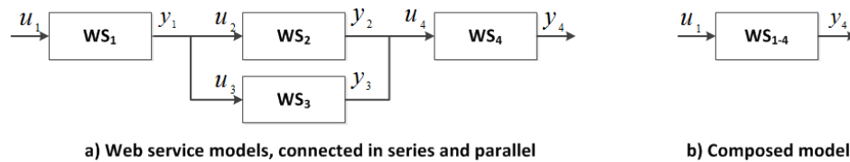
Fig. 9. Model composition for web services.
