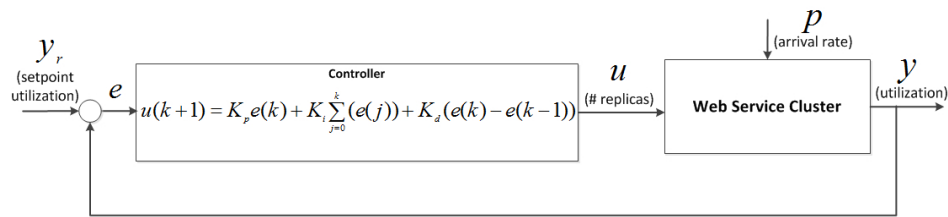
Fig. 8. A feedback loop with a PID controller for distributing the web service load in a cluster.
