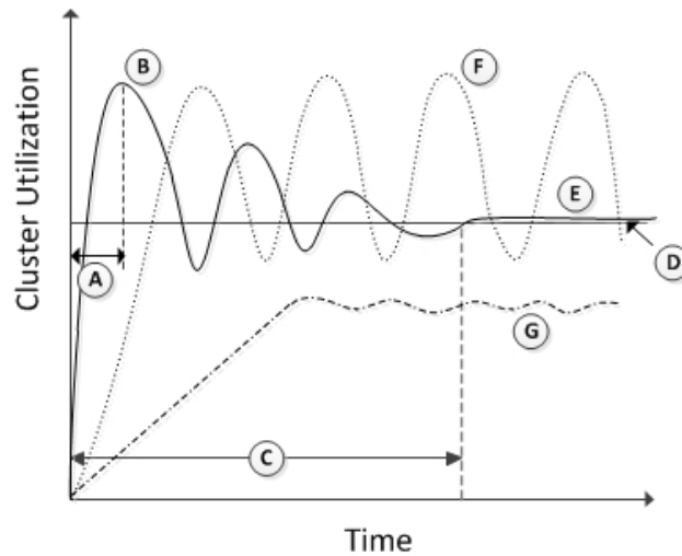
Fig. 10. Quality metrics for a controlled system [6]: rise time (A); overshoot (B); settling time (C); steady error or accuracy (D). Fine-tuned values for a PID controller, K_p, K_i, K_d , result in a smooth behavior reaching the reference level with accuracy and acceptable settling time (curve labeled (E)). Large values for K_p (and in lesser extents K_i and K_d ), produce corresponding large oscillations around the reference level (curve labeled (F)). Small values usually result in a sluggish behavior (curve labeled (G)).
